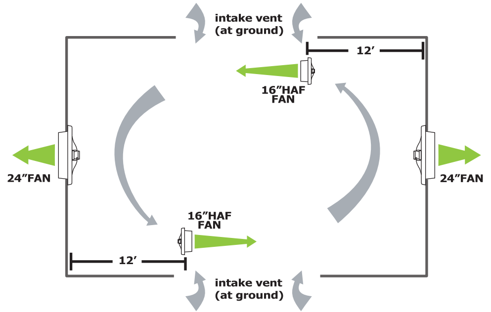
36'x24' Greenhouse
