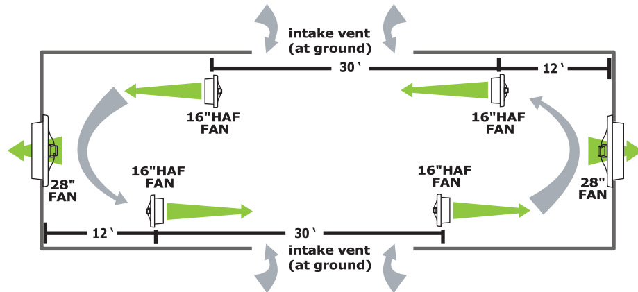
60'x20' Greenhouse
