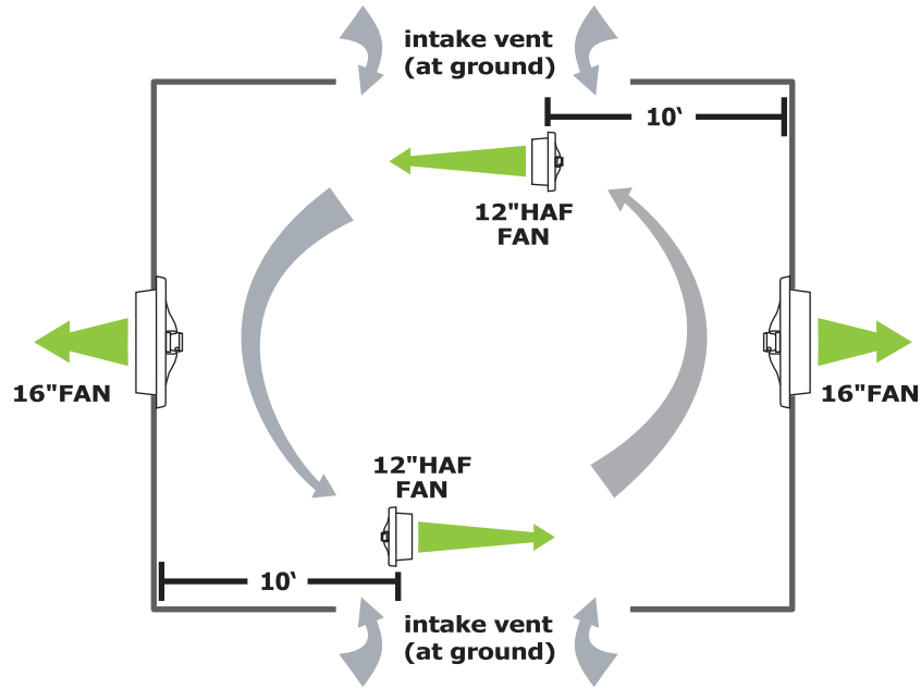
24'x20' Greenhouse
