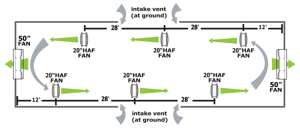
96'x30' Greenhouse
